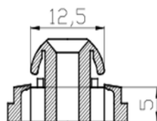
Clip automatica marrone sp.5mm
